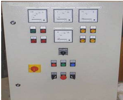
MCC PANEL
